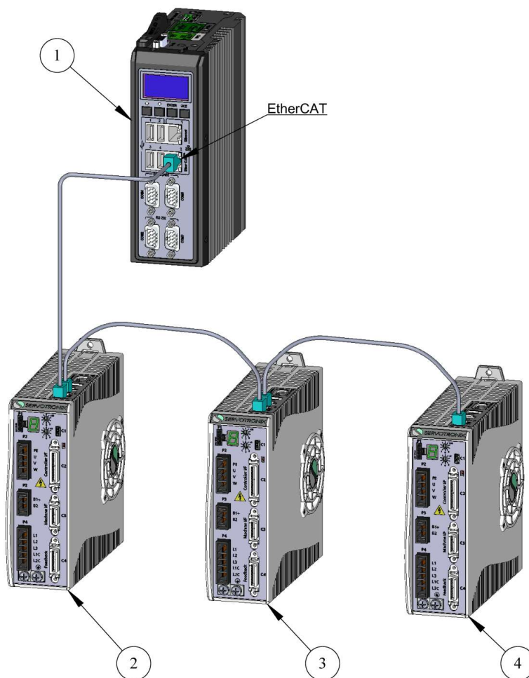
Figure 2-4. FLEXI PRO – EtherCAT Configuration – softMC 7 Controller – Example
