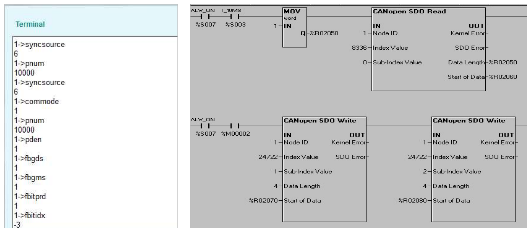
Figure 4-13. Parameter Settings in Flexi SUITE and in Cscape
