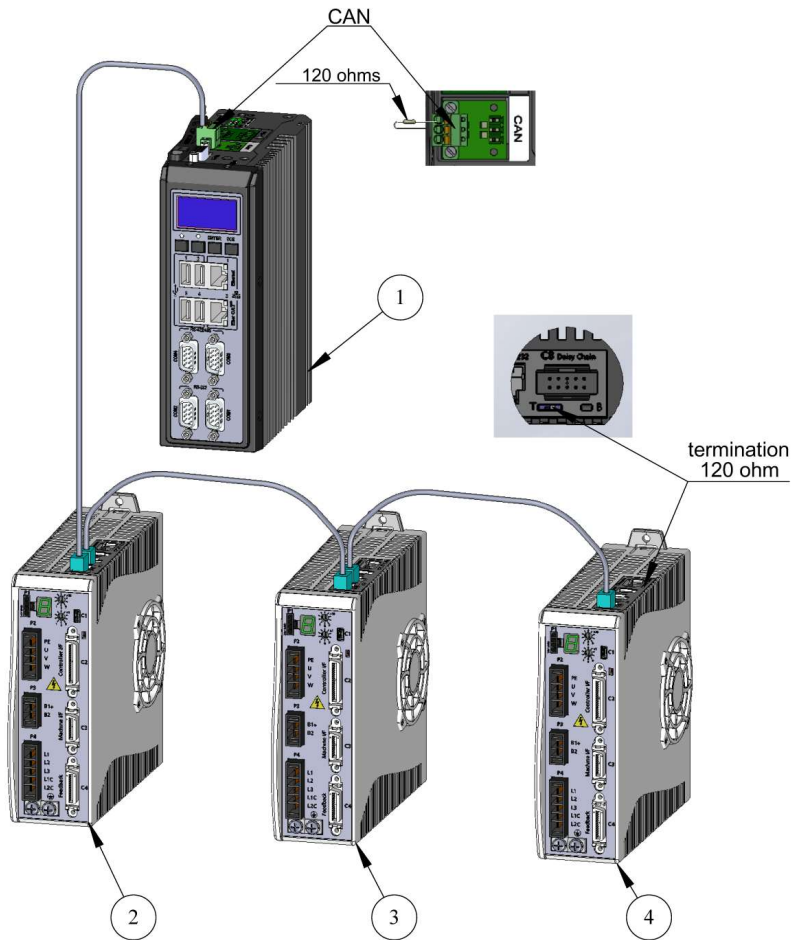
Figure 2-1. FLEXI PRO – CAN Configuration – softMC 7 Controller – Example
