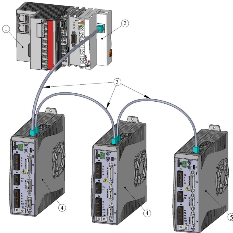
Figure 2-5. FLEXI PRO – EtherCAT Configuration – Beckhoff Controller – Example
