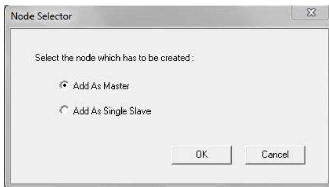
Figure 4-5. Node Selector
