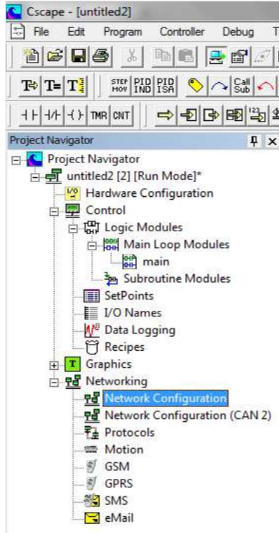
Figure 4-4. Project Navigator
