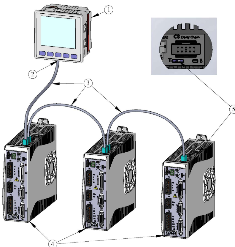
Figure 2-2. FLEXI PRO–CAN Configuration – Horner Controller – Example
