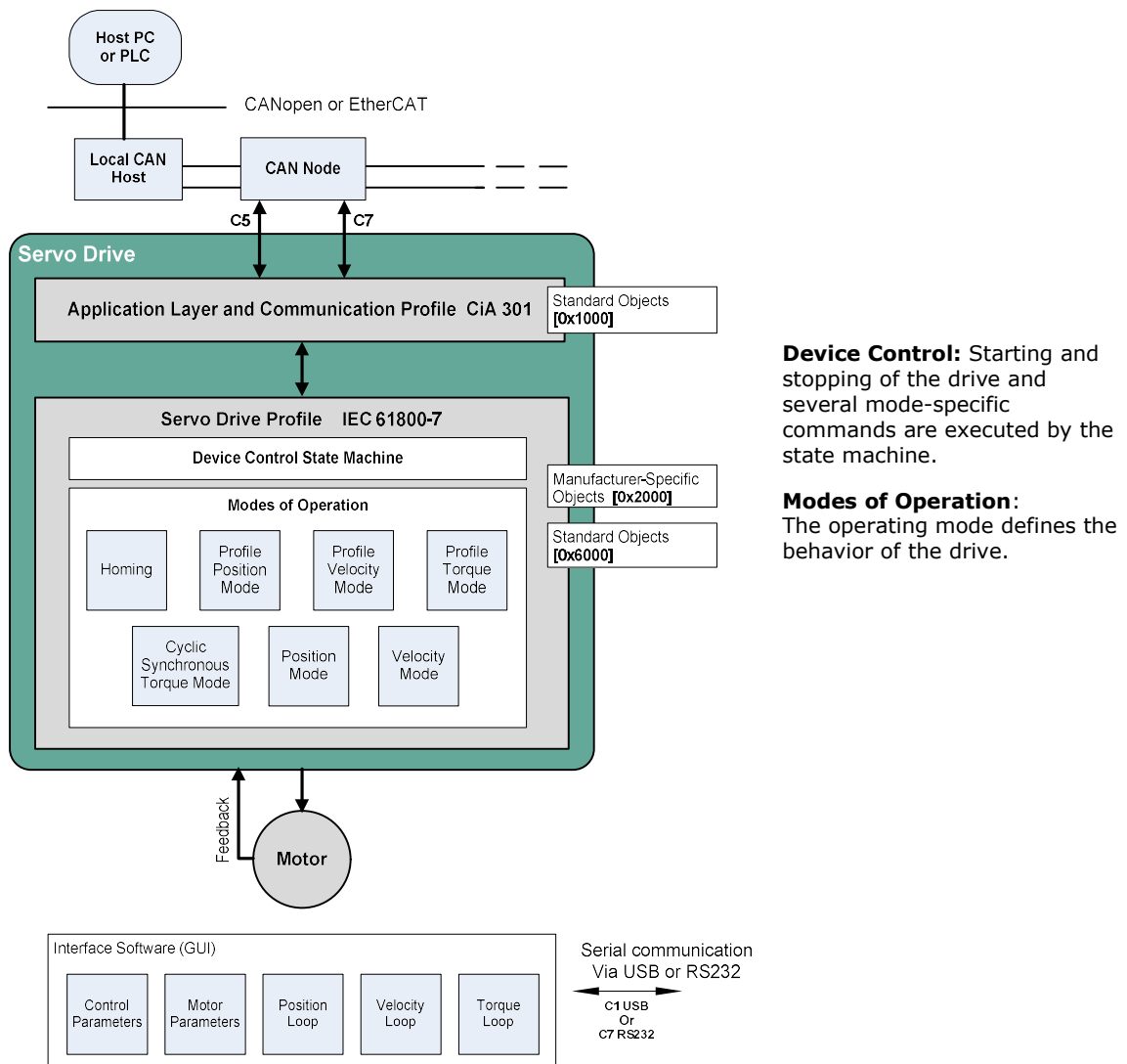
Figure 7-1. Communication Architecture
