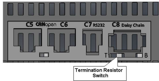
Figure 2-7. FLEXI PRO Termination resistor switch
