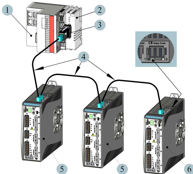
Figure 2-3. FLEXI PRO – CAN Configuration – Beckhoff Controller – Example
