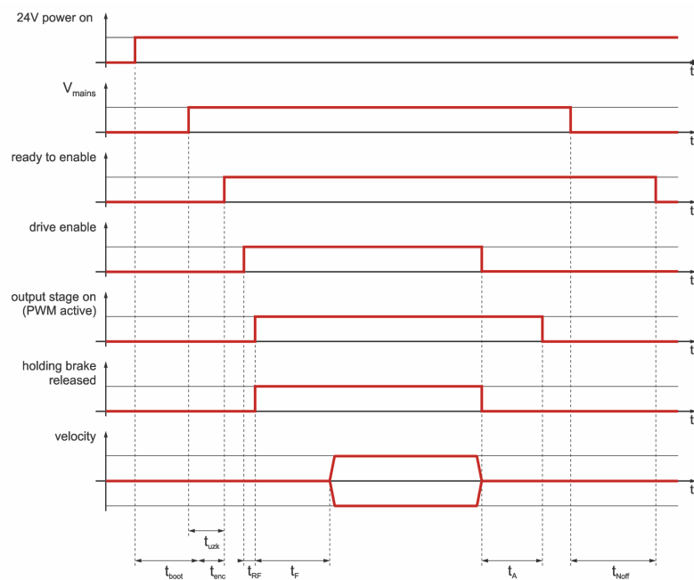
Figure 26: Time diagram of the servo drive
