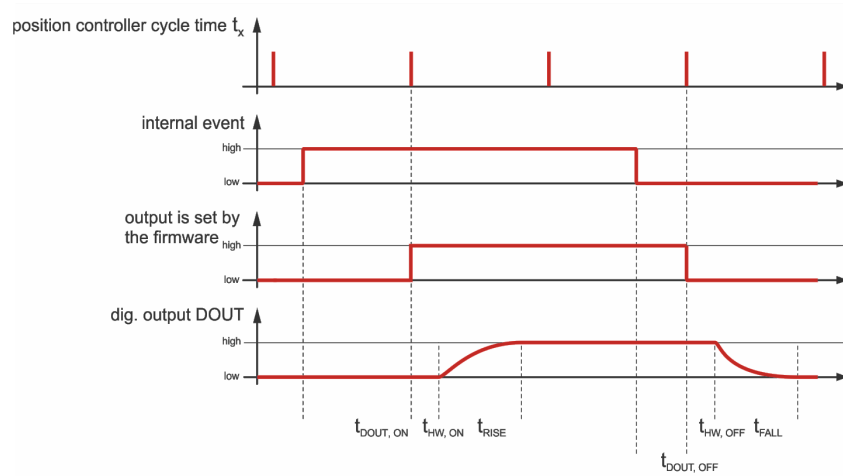
Figure 25: Filter time mechanism in the case of digital outputs
