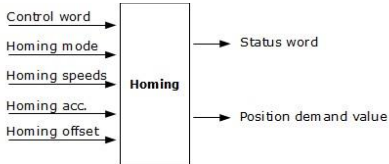
Figura 4: Homing function
