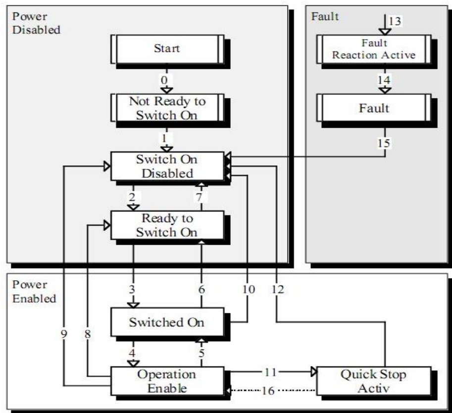
Figura 19- State Machine
