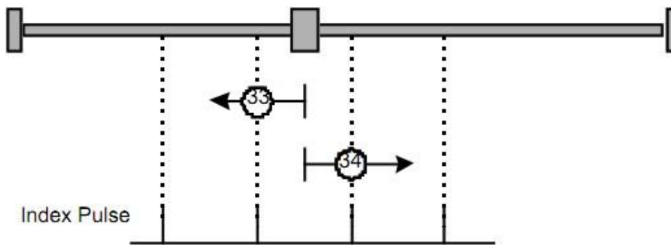
Figura 12 Homing on index pulse
