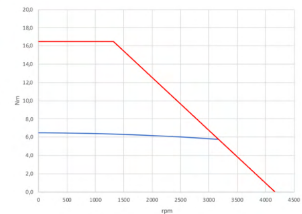
Operative curves at 48 Vdc
