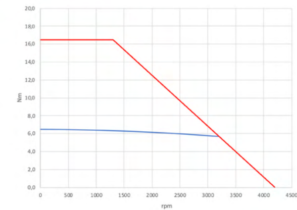
Operative curves at 96 Vdc
