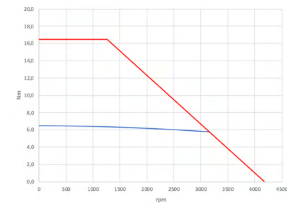
Operative curves at 72 Vdc
